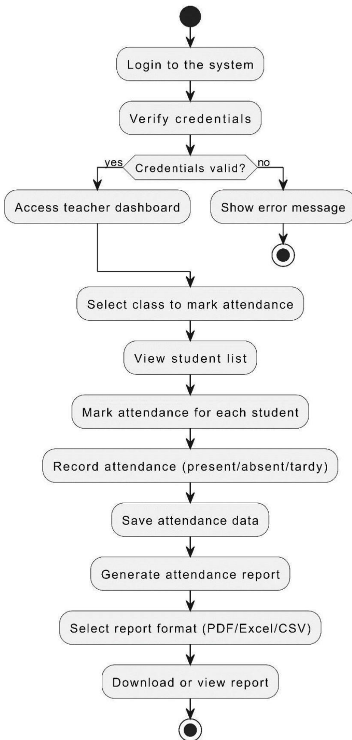
Figure 6:Activity diagram of E-Class
